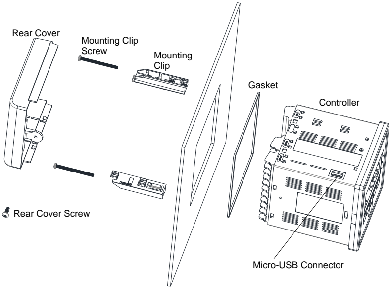
Figure 1 Exploded View
