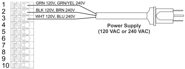
Figure 12 P120 AC Power & Relay Output Wiring
