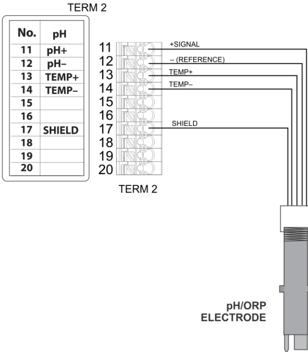
Figure 7 Non-Amplified pH/ORP Sensor Input Wiring
