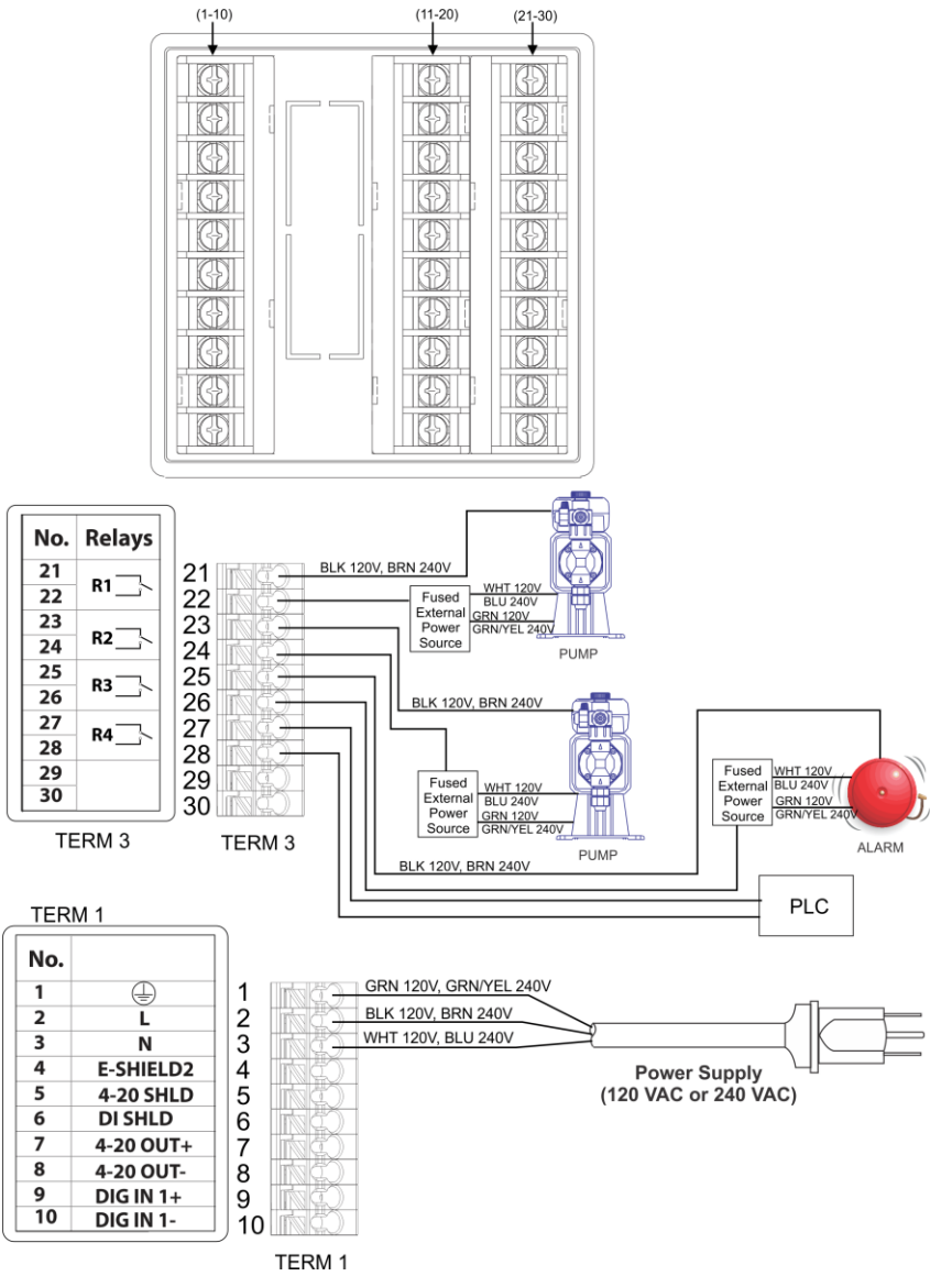
Figure 11 P110 AC Power & Relay Output Wiring
