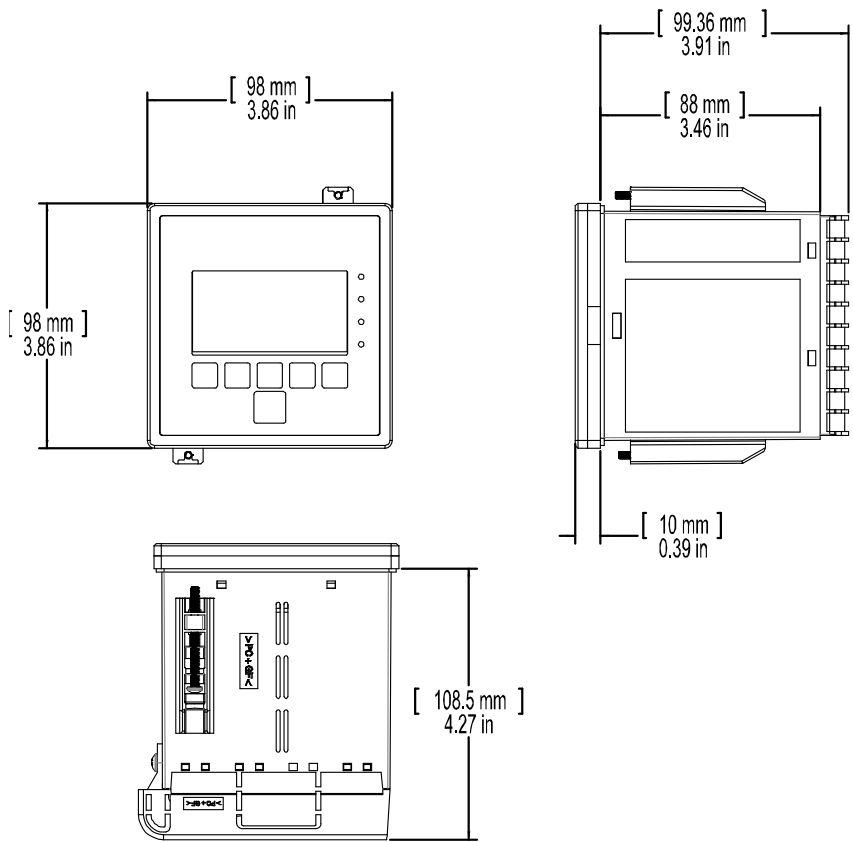
Figure 3 Controller Dimensions
