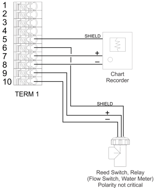
Figure 10 Digital Input /Analog Output Wiring
