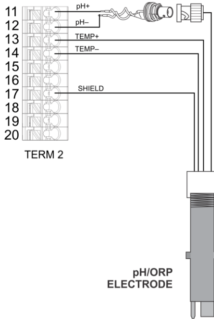
Figure 6 Non-Amplified pH/ORP Sensor Input Wiring with BNC
