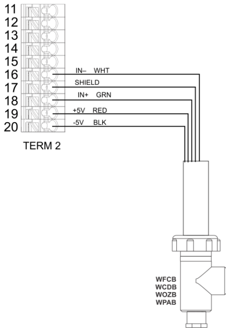
Figure 9 Disinfection Sensor Input Wiring
